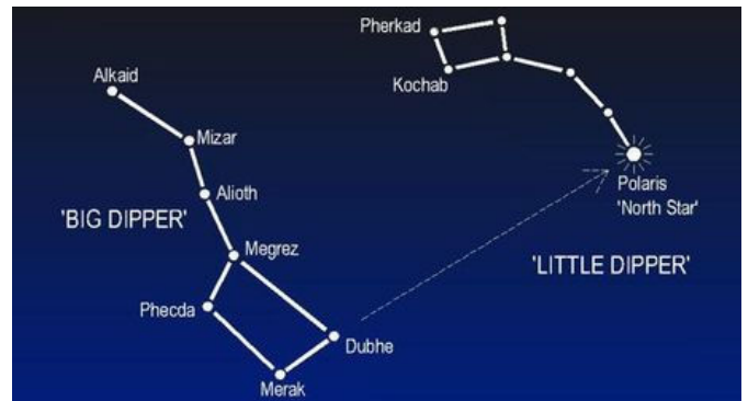
Figure 4 - Big Dipper and Little Dipper
